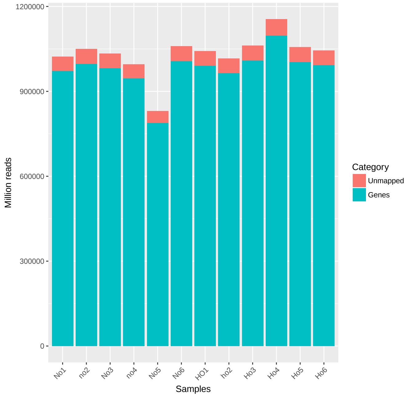
Read counts
