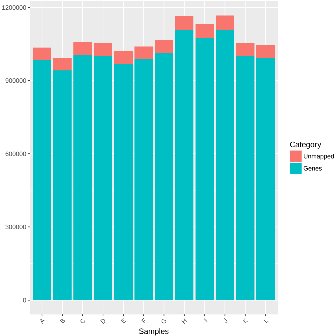
Read counts
