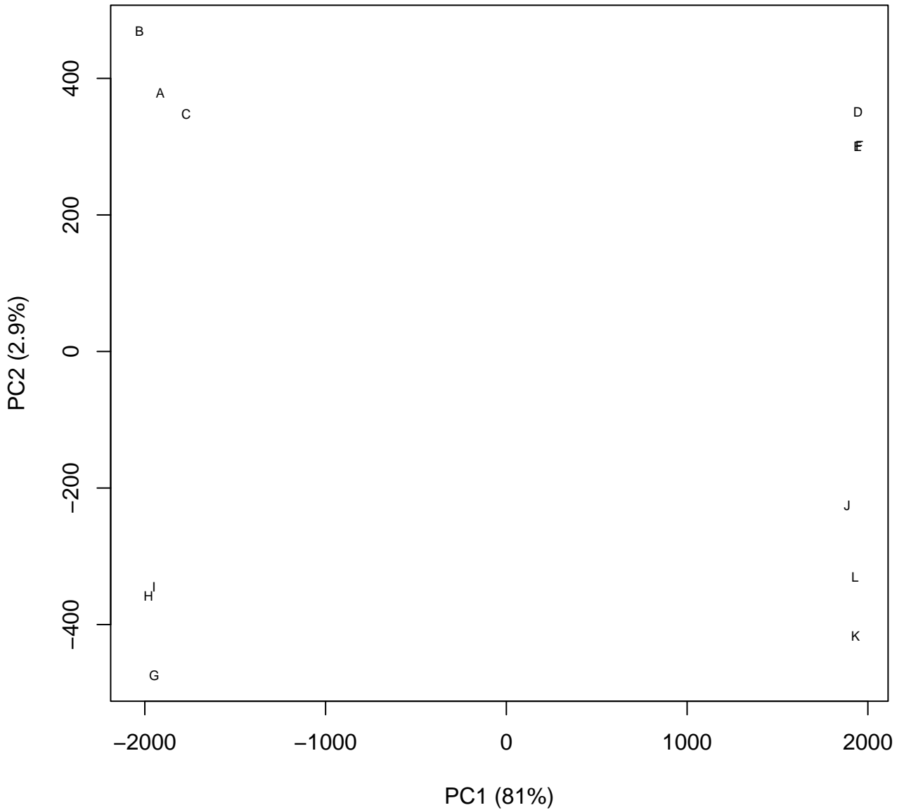
PCA plot: Sample Names
